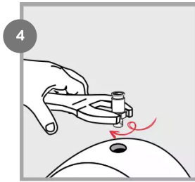
Screw BSP 1/8 fitting on lube point.
