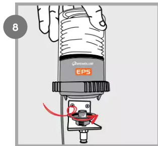
Install MEMOLUB EPS Series lubricator on Memo. Connect the cable to the 24V DC power supply.
