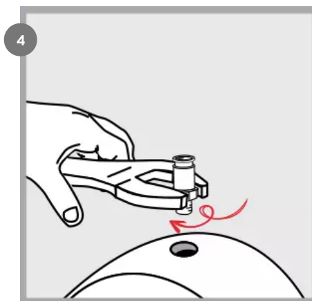
Install BSP 1/8 fitting on lube point.
