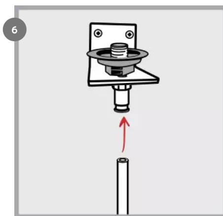
Insert hose into the bracket's quick fitting.
